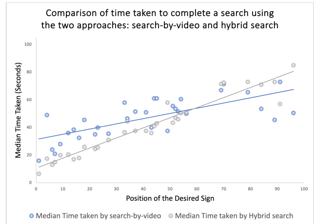
Figure 4: Scatterplot displaying median search times, for each rank-position on the search-results page, for the hybrid-search and search-by-video prototypes, and with best-fit lines added for each group.
